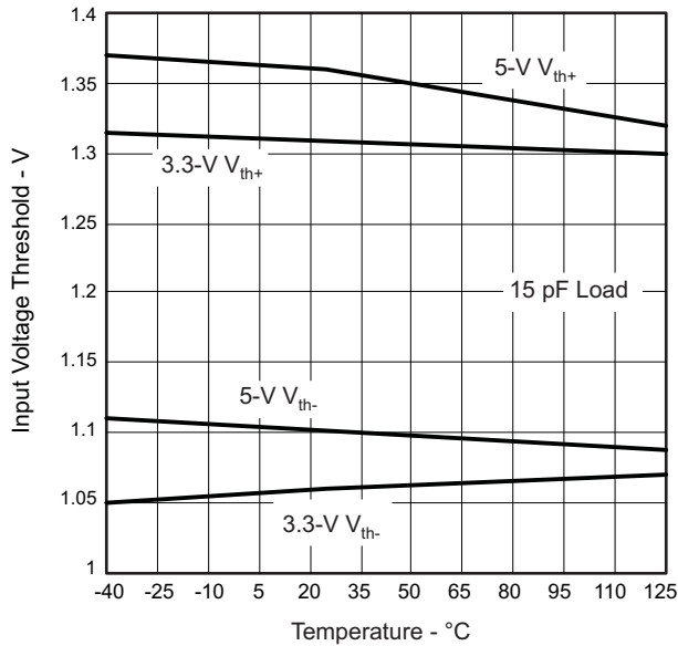
ISO722xA AND ISO722xC INPUT VOLTAGE LOW-TO-HIGH SWITCHING THRESHOLD vs FREE-AIR TEMPERATURE
