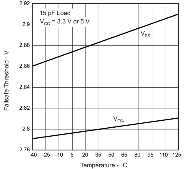
V CC FAILSAFE THRESHOLD vs FREE-AIR TEMPERATURE
